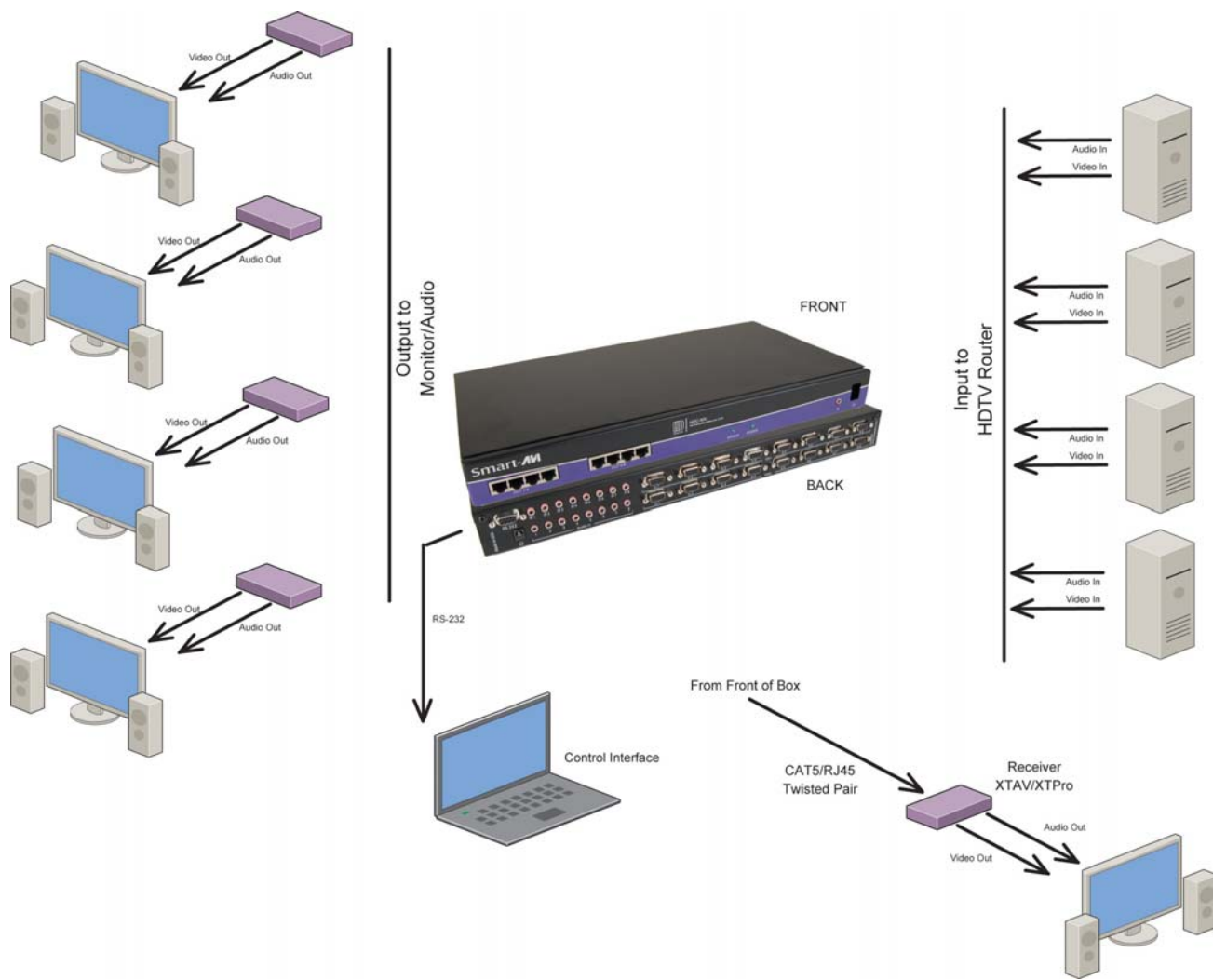
HDTV Router connection diagram
