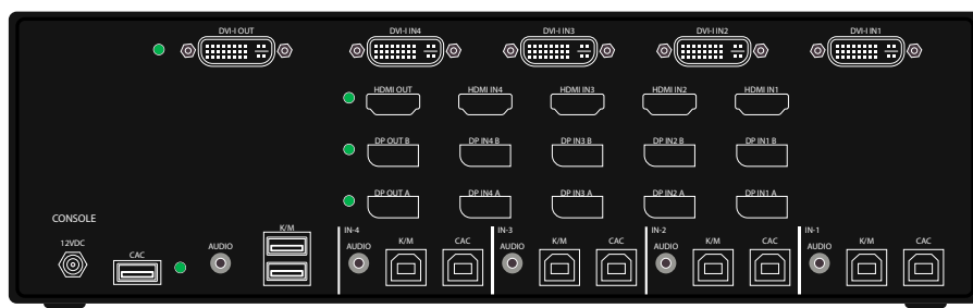
Figure 4-2: SA-DPH-4Q-P Rear panel
