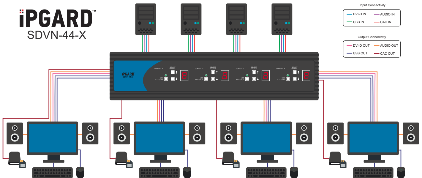
Figure 7-1: SDVN-44-X
