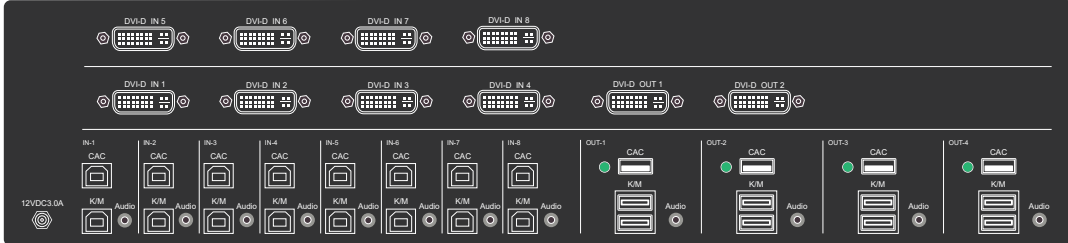
Figure 5-4: SDVN-82-X Rear panel
