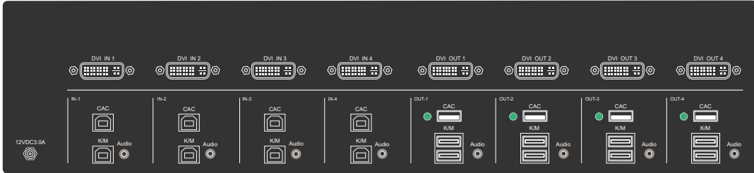
Figure 5-2: SDVN-44-X Rear panel
